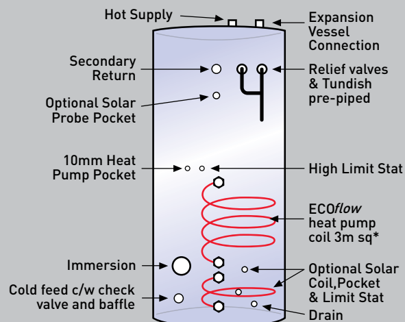
ECOflow Schematic (with optional solar coil)
